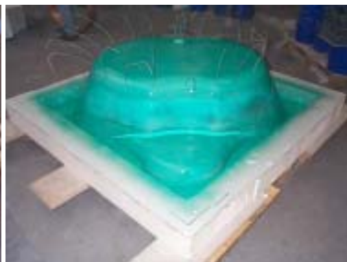
pattern with releaser and vacuum wires
